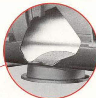
Filtorr separator is mounted contour to the shape of the mixer shell allowing minimum clearance between the mixing plows and the Filtorr media.
